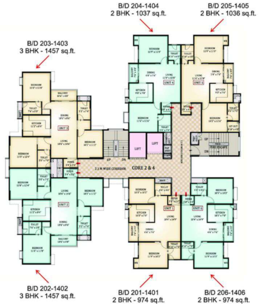
Core 2 & 4 - Typical Floor Plan
